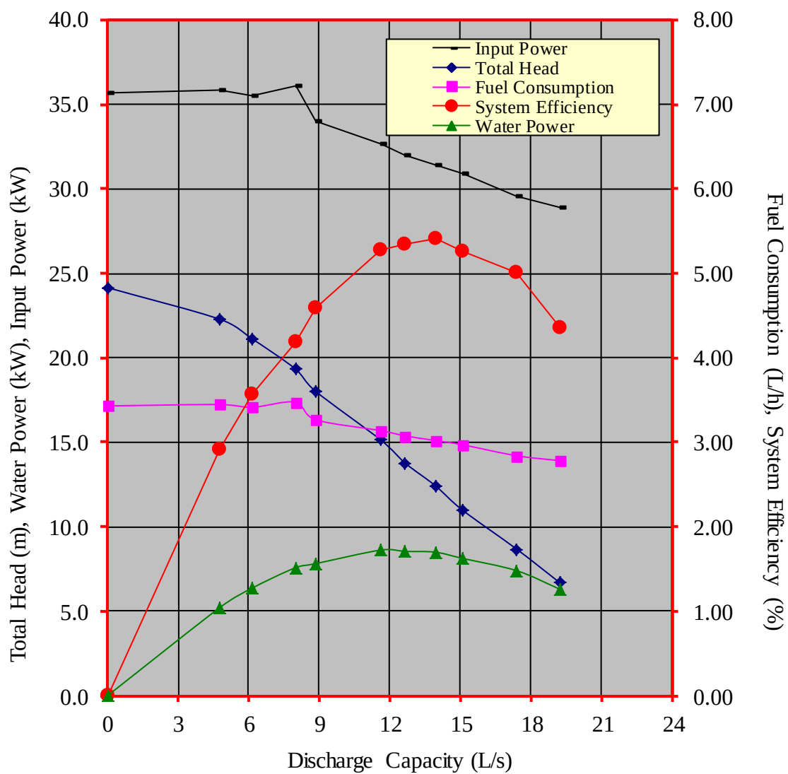
Figure 3. Performance characteristic curves of the MIYATA NS-100 centrifugal pump coupled to TARO TS80RE diesel engine
