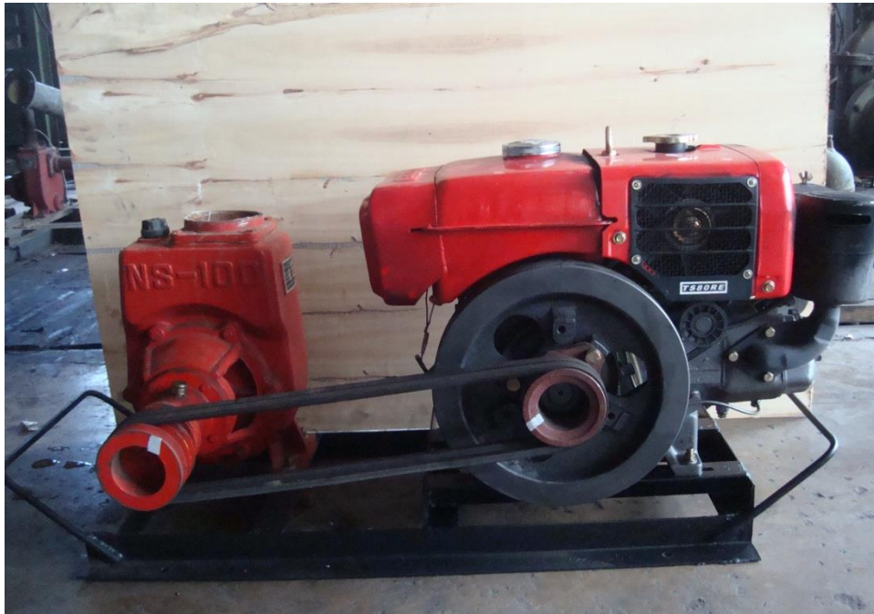
Figure 2. MIYATA NS-100 Centrifugal Pump coupled to a TARO TS80RE Diesel Engine
